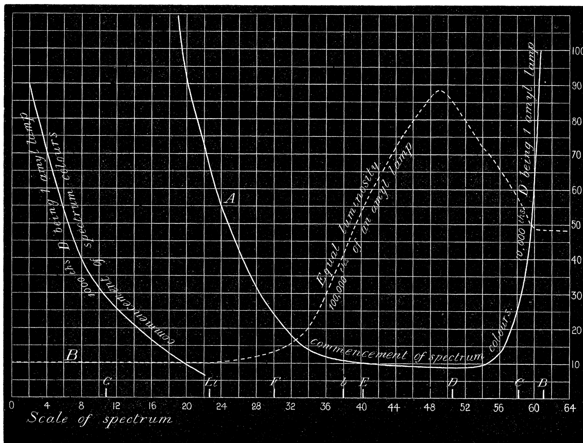
Diagram of limit of colour vision.
